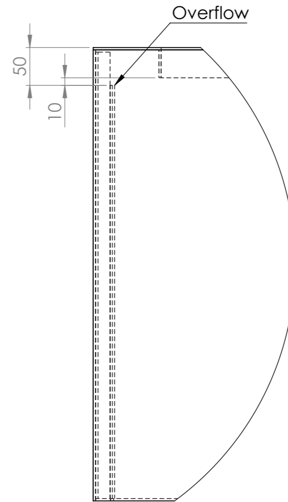
DETAIL C SCALE 1 : 5
