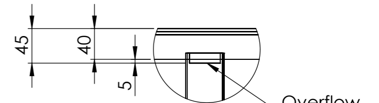
DETAIL B SCALE 1 : 5
