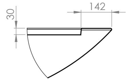
DETAIL 2 SCALE 1 : 10
