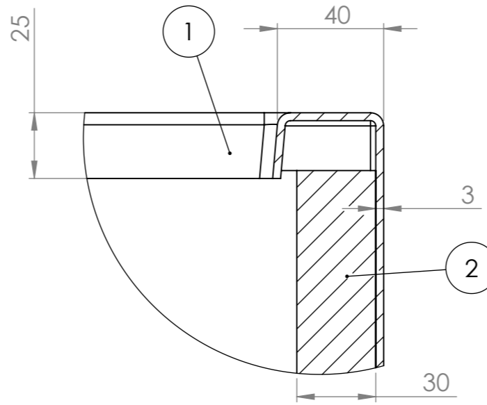
DETAIL B SCALE 1 : 2
