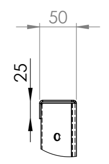
DETAIL A SCALE 1 : 5
